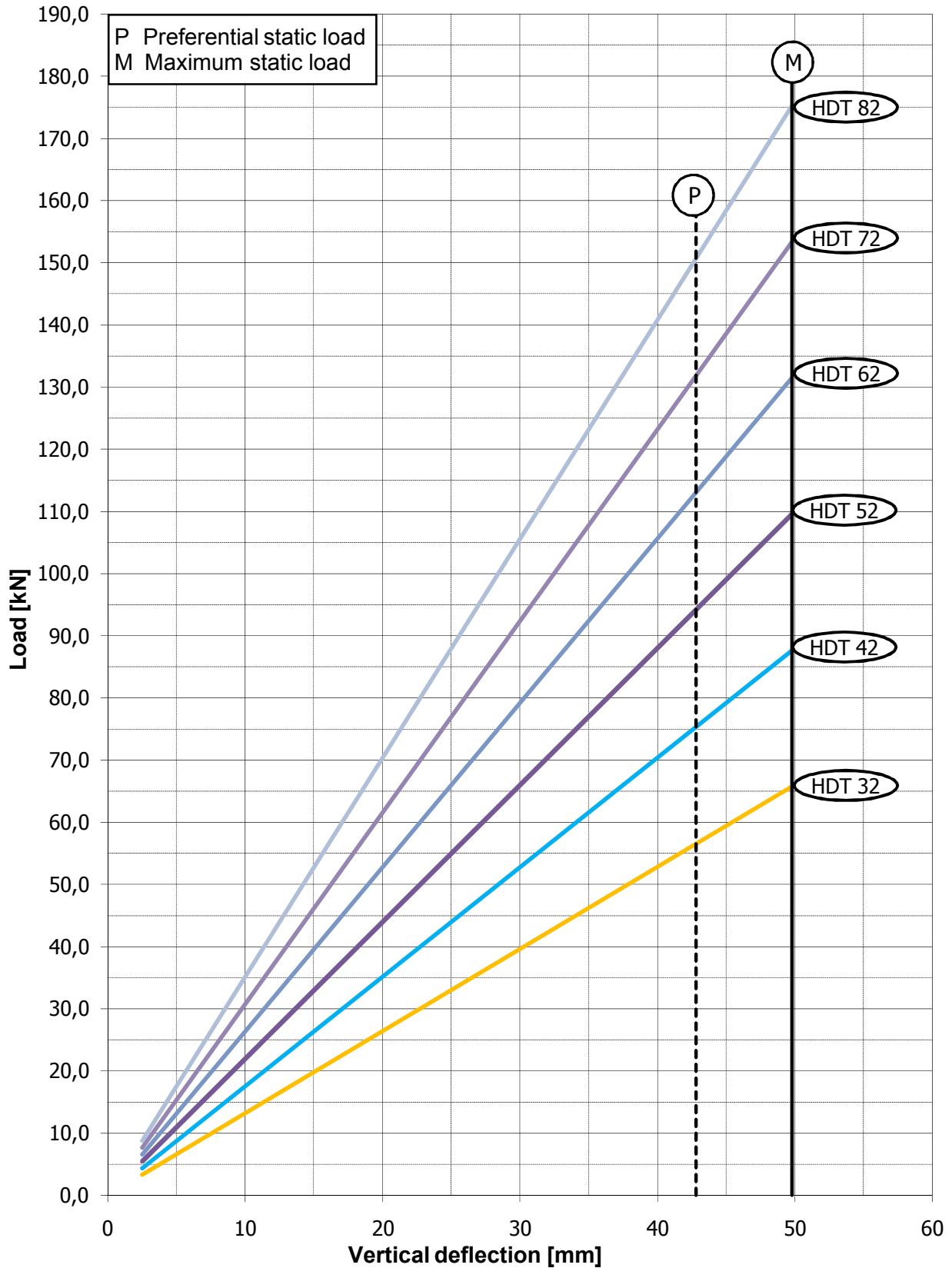
Vertical load / deflection characteristics HDT2
