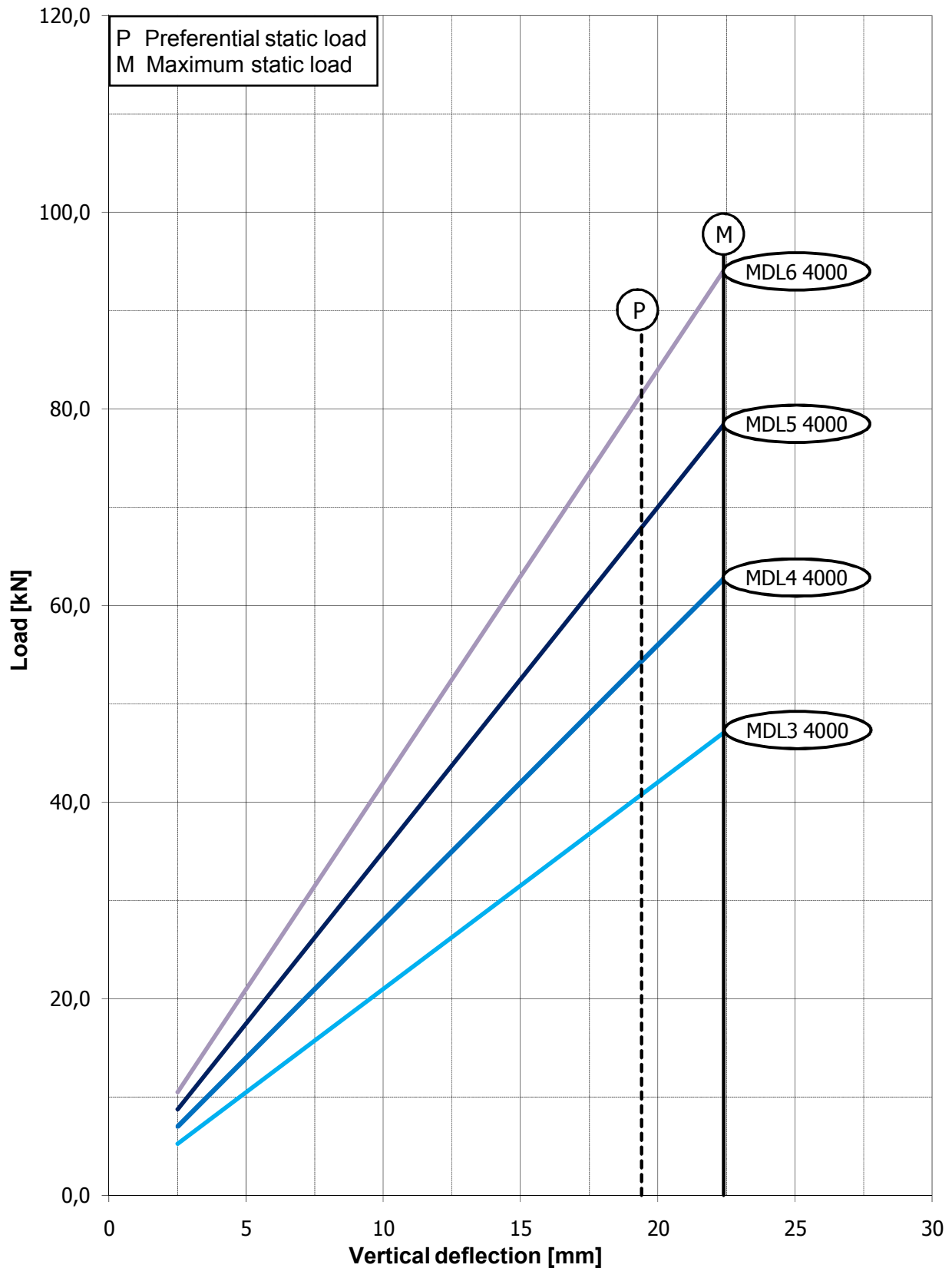
Vertical load / deflection characteristics MDL 4000
