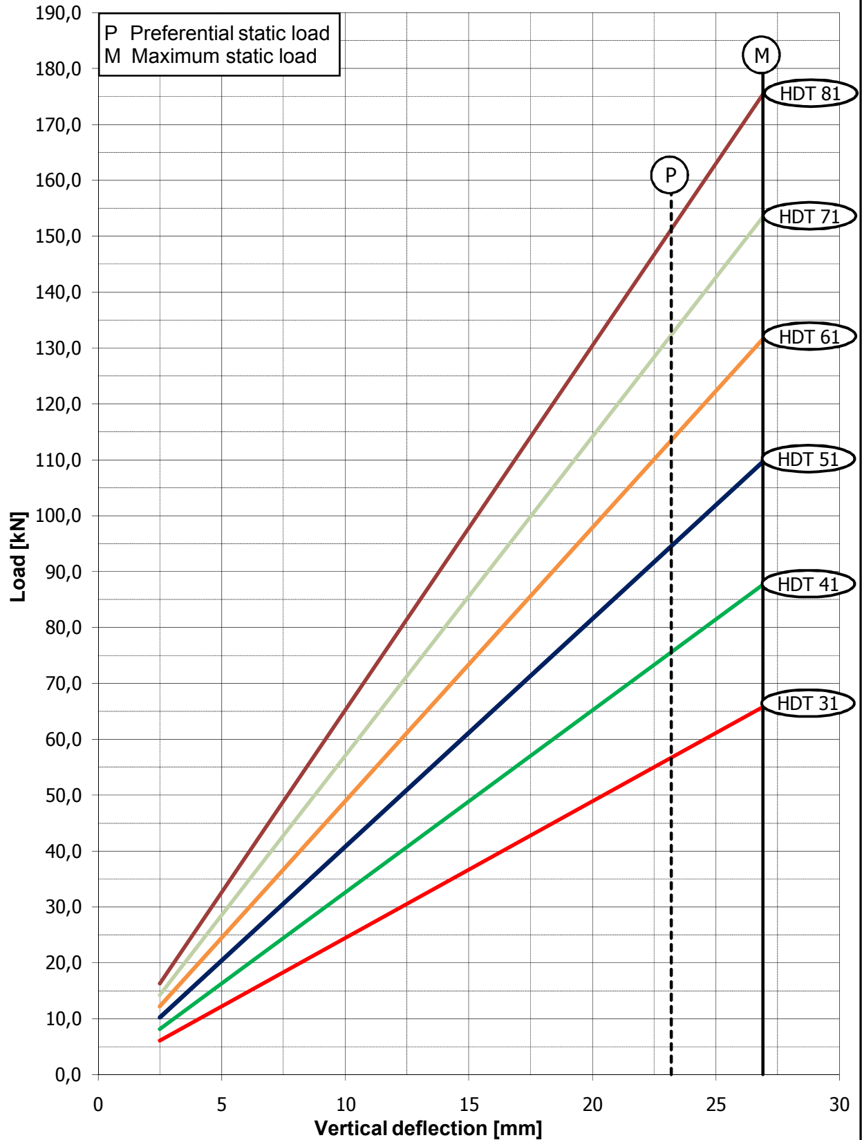
Vertical load / deflection characteristics HDT1
