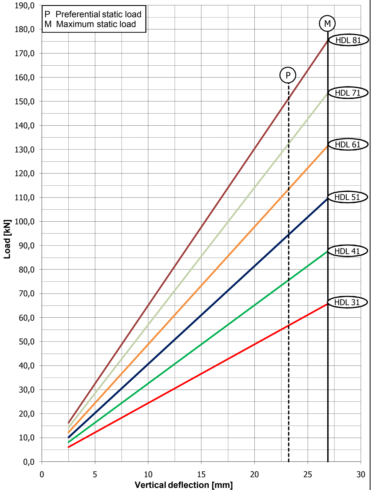
Vertical load / deflection characteristics HDL1
