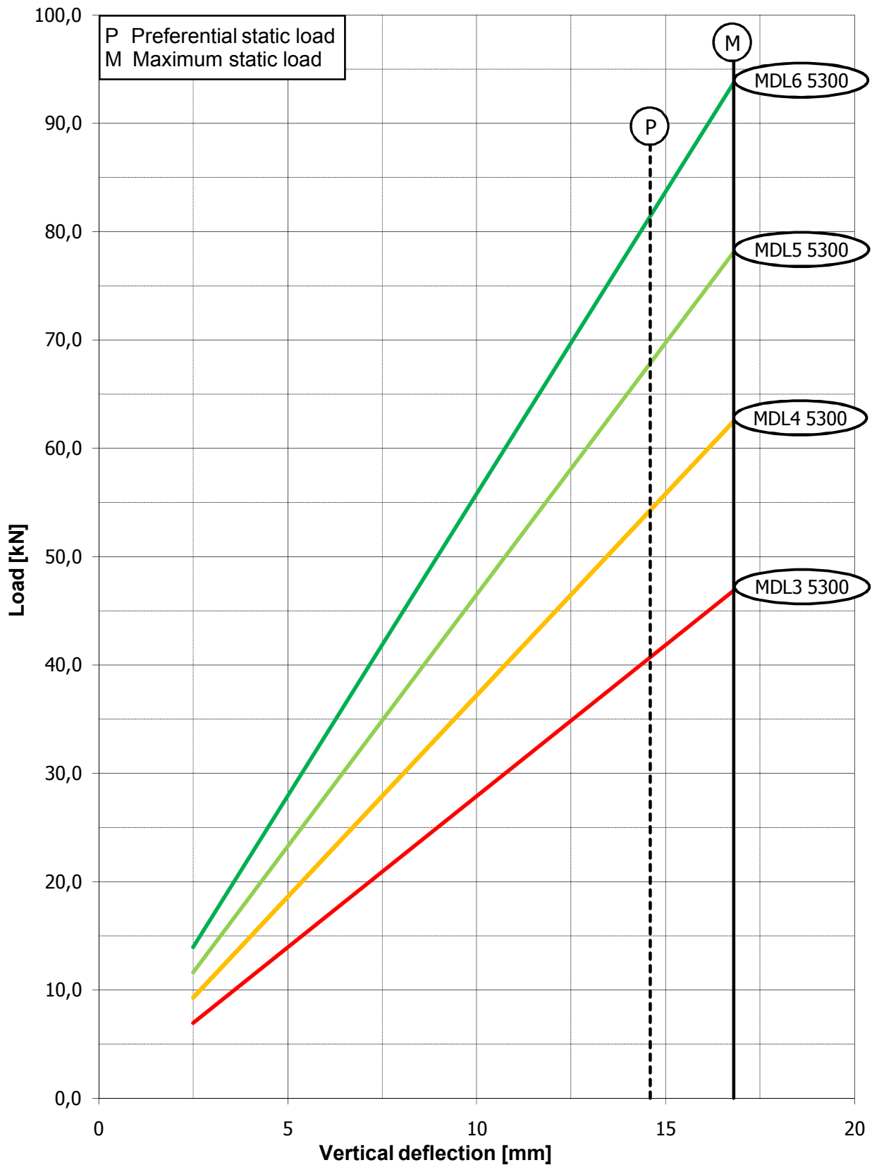
Vertical load / deflection characteristics MDL 5300
